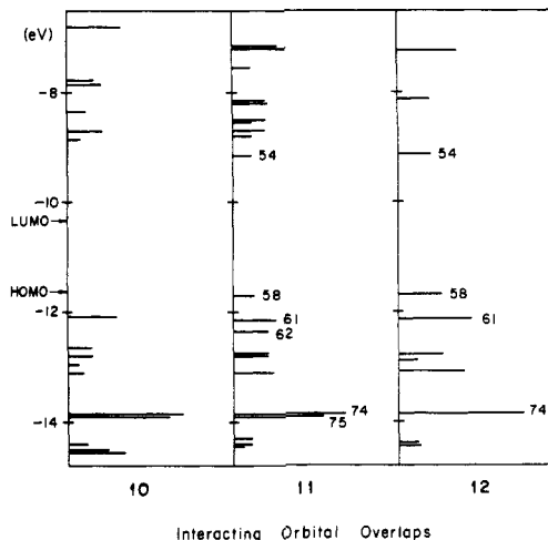
Figure 2. Interacting orbital overlaps of the carbide orbitals with a model hydrogenic wave function for the structures 10–12. The HOMO and LUMO shown are for Fe_5(CO)_{15}C . Numbering for the butterfly cluster corresponds to Figure 1.
