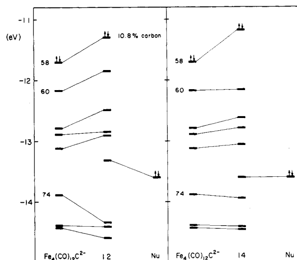
Figure 4. Interaction of a model nucleophile ( H_{ii} = -13.6 eV) with the butterfly carbide: left, attack on carbon, 12 ; right, attack on the back Fe-Fe bond, 14 . Only orbitals of a_1 symmetry are shown.
