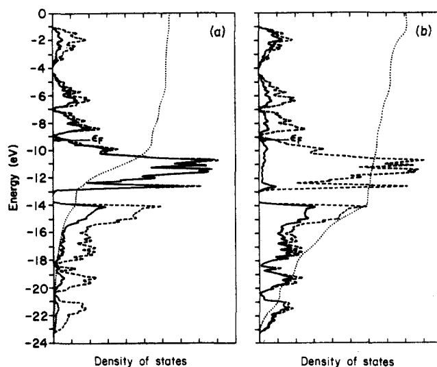
Figure 13. Contributions of (a) metal and (b) phosphorus orbitals to the total DOS for the NiP lattice. The dashed line is the total density of states, and the dotted line is the integration curve. The Fermi level for NiP is marked by an arrow.
