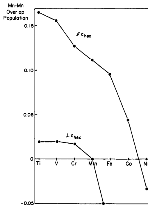
Figure 9. Metal-metal overlap populations as a function of the electron count in the NiAs type lattice: (a) for metal chain parallel to c_{hex} and (b) for metal-metal contacts perpendicular to c_{hex} .
