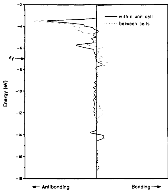
Figure 3. Crystal orbital overlap population of the Cu-Cu bonds for the one-dimensional Cu chain (a) and the two-dimensional Cu 2 Ga layer (b). In the latter case we have to consider the Cu-Cu bonds within the unit cell (Ga-bridged Cu atoms) and between neighboring unit cells.
