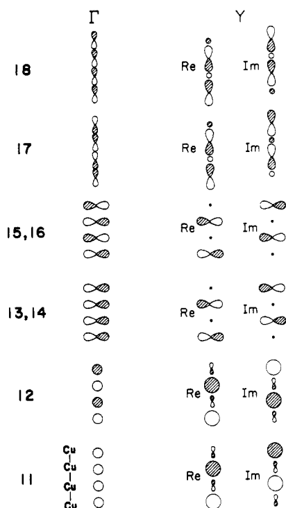
Figure 2. Orbital compositions of the bands 11-18 for the equidistant one-dimensional Cu chain. We have included two unit cells, i.e. four Cu atoms. At Y we show the real part (Re) and the imaginary part (Im) of the wave function.
