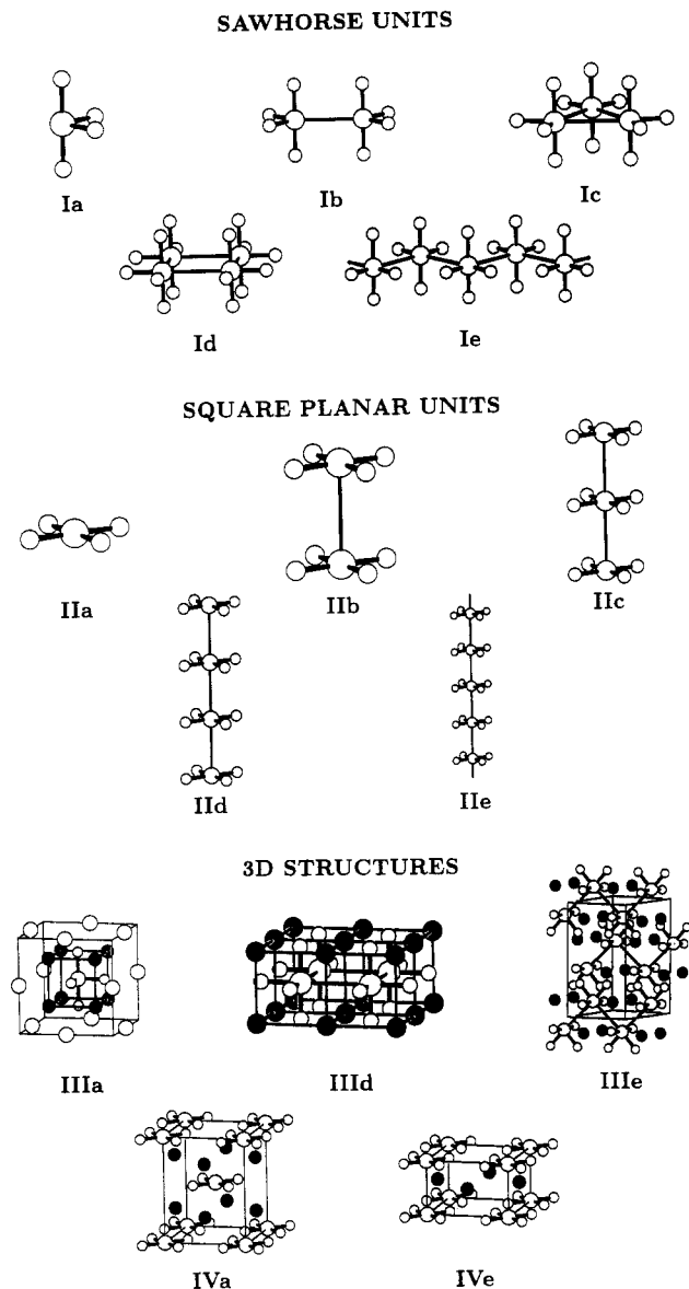
Figure 1. Structural models listed in Table 1. Small shaded circles are Mg and Na; large open circles are Ru and Pt; small open circles are H.
