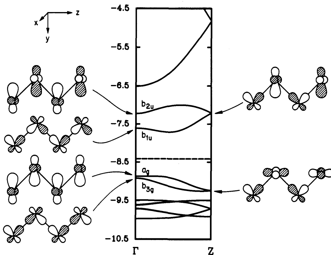
Figure 3. Energy bands of \text{Mg}_2\text{RuH}_4 along the \Gamma\text{Z} line in the orthorhombic Brillouin zone (parallel to c^* ). The dashed line at -8.4 eV is the calculated Fermi level. Crystal orbitals at \Gamma and \text{Z} for the highest occupied, b_{3g} and a_g , and lowest unoccupied bands, b_{1u} and b_{2u} , are also depicted.
