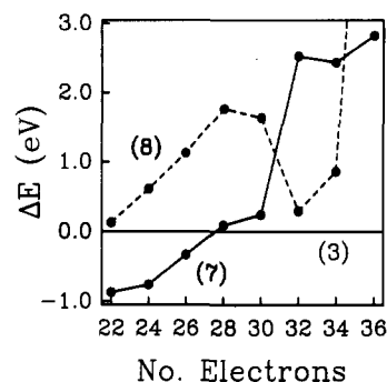
Figure 6. Energy difference curves between three models of \text{Ru}_2\text{H}_6 : solid line, square planar dimer 7 ; dashed line, tetrahedral dimer 8 . The reference geometry is the dimer of T-fragments ( 3 ). Lowest line corresponds to most stable geometry.
